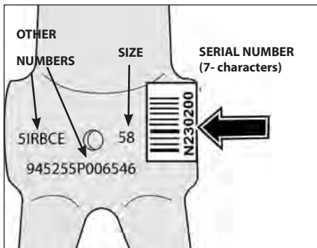
Figure 29. Underside of Bottom Bracket
